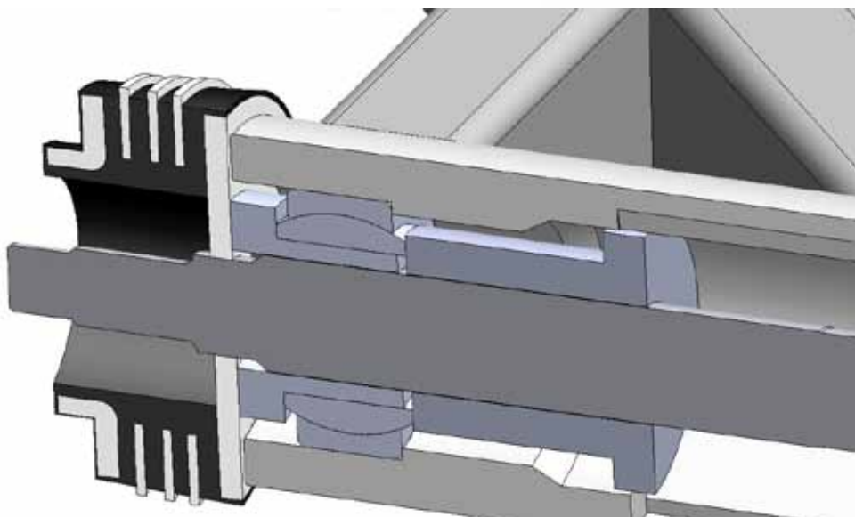
Figure 5 Close up Sectional view of Pivot Shaft Assembly
