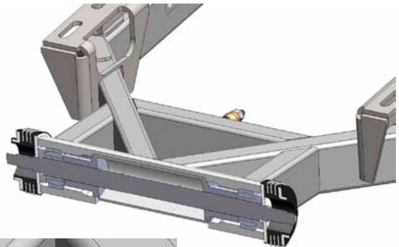
Figure 5 Sectional view of Pivot Shaft Assembly
